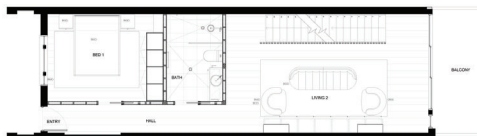
Ground Floor
